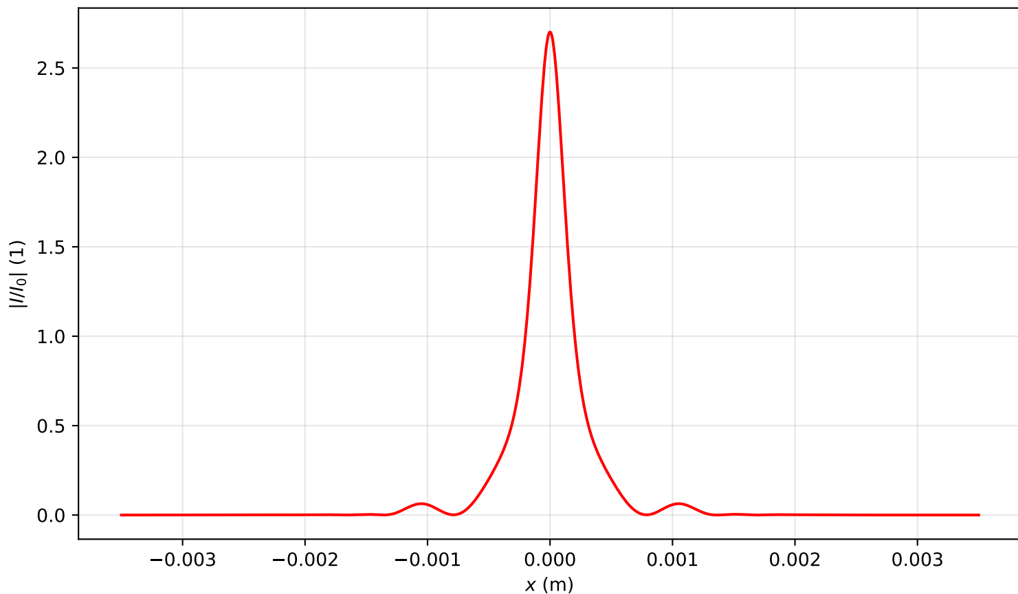
Intensity profile I(x, y = 0, z = 1.672)/I_0 , P_{in}=2.5P_{cr} , artificial time
